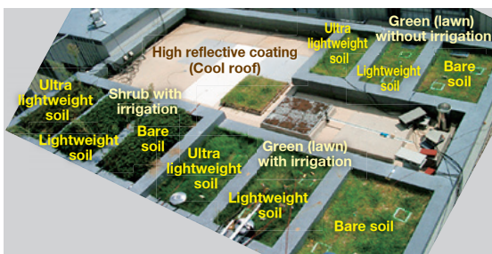
Experimental roof for surface cover technology in an urban structure at Kobe University (Study on urban thermal environment by Assoc. Prof. Takebayashi)
