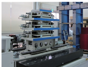
Shaking table
