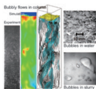
Fig. 1 Multiphase Fluid Dynamics
