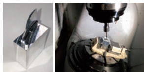
Fig. 3 High speed and high precision machining of parts for jet engines
