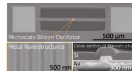
Fig. 4 Optical sensor for large capacity information communication
