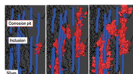
Fig. 2 CT imaging of corrosion fatigue crack initiation process
